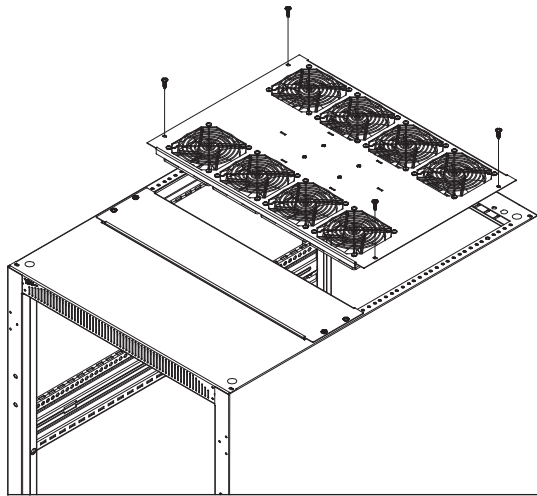
(I)BGR-552FT/(I)BGR-552FT-FC MODELS
