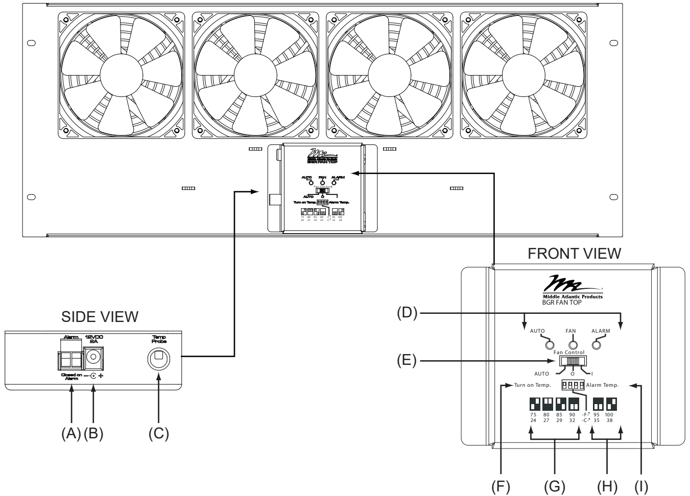
(I)BGR-276FT-FC SHOWN
