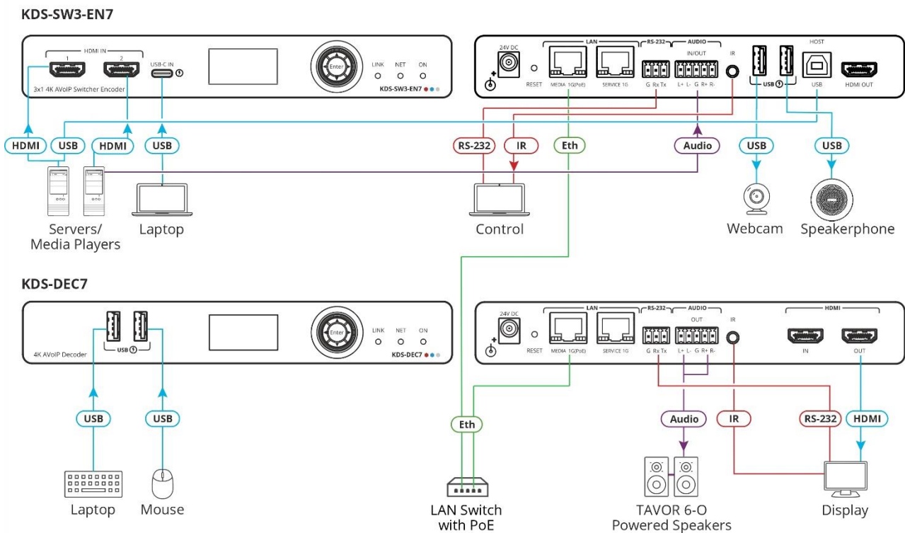
Figure 2: Connecting the KDS-SW3-EN7 and KDS-SW3-EN7
