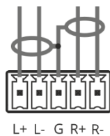
Figure 3: Connecting to a Balanced Stereo Audio Source/Acceptor
