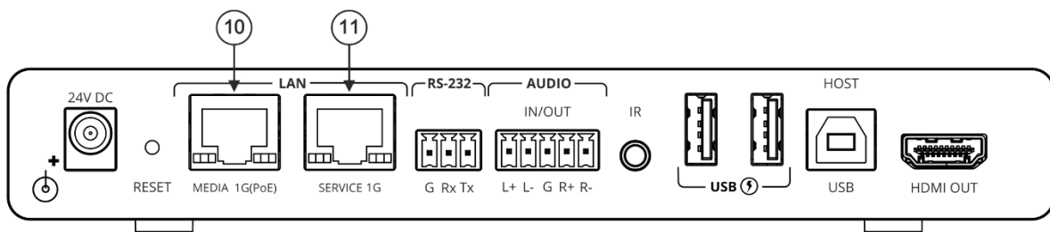
Figure 24: Ethernet ports on the rear of the KDS-SW3-EN7
