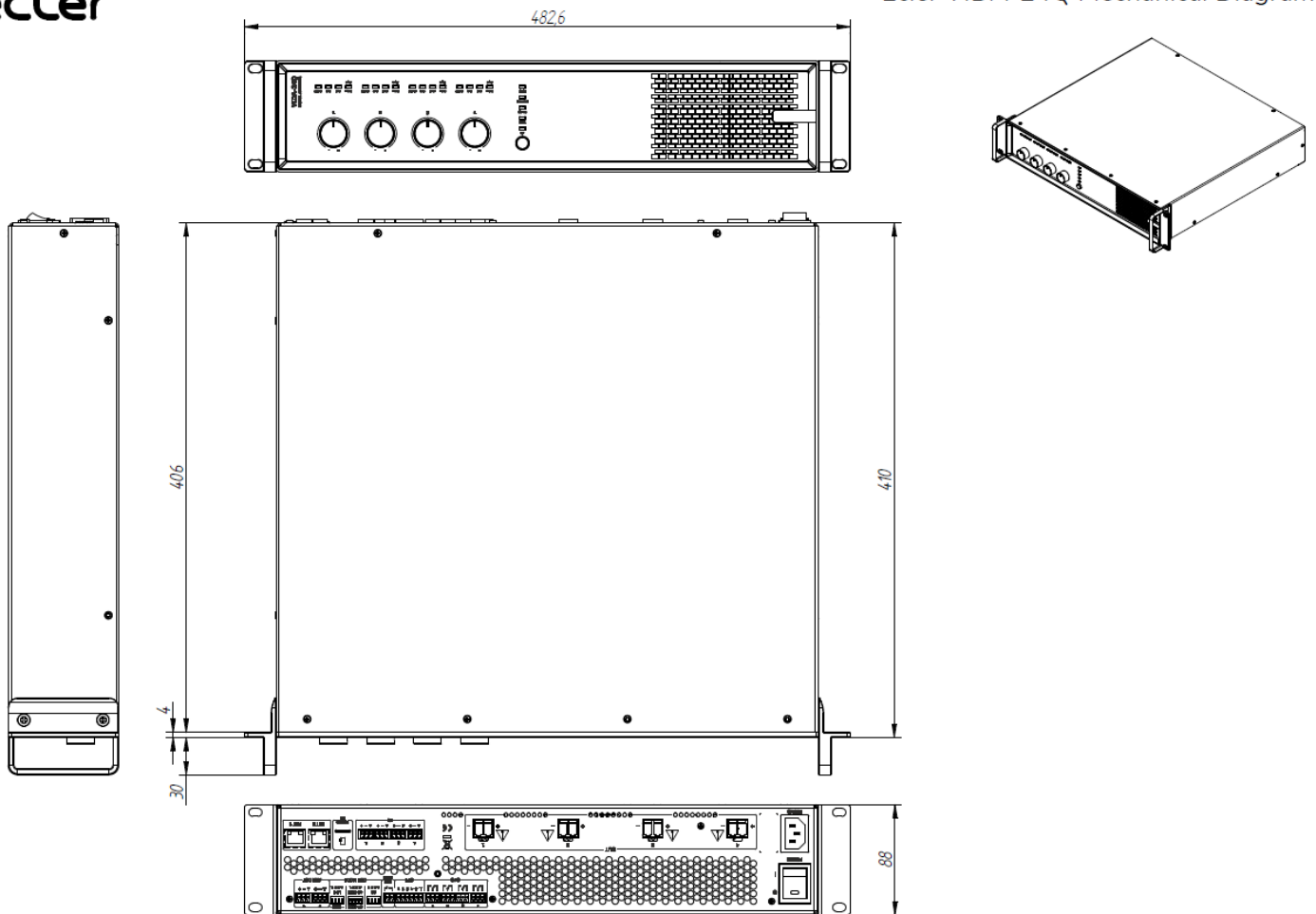
Ecler VIDA-24Q Mechanical Diagram
