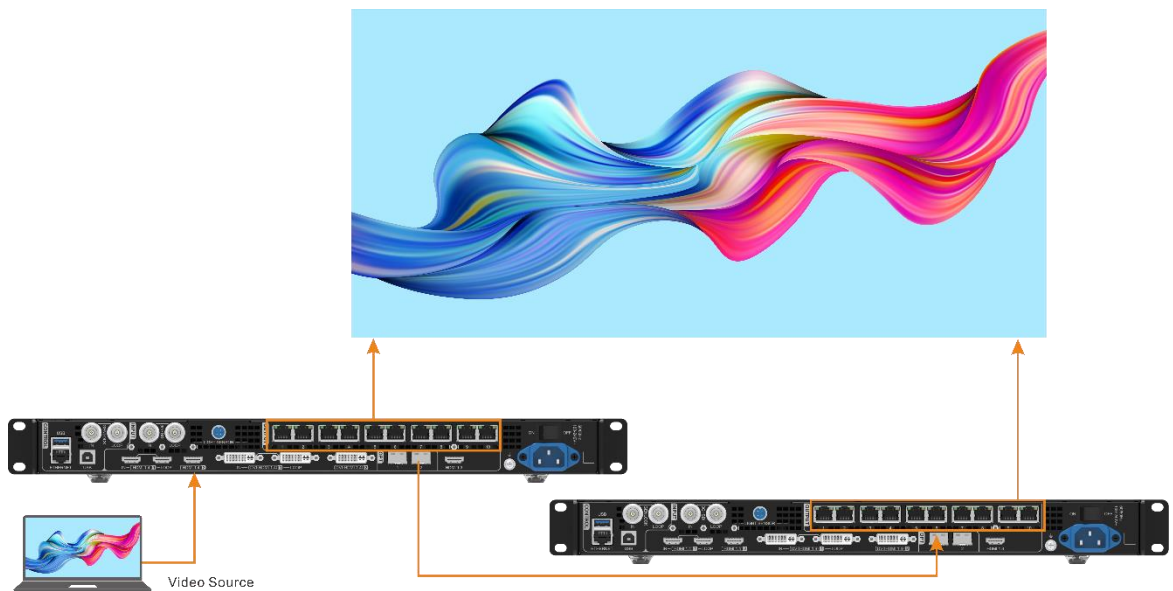
Figure 5-43 Backup
