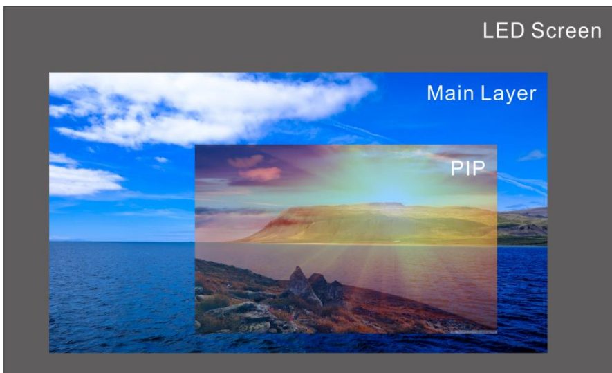
Figure 5-15 Opacity
