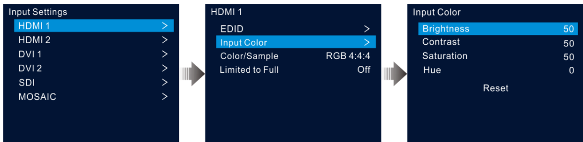
Figure 5-19 Input color
