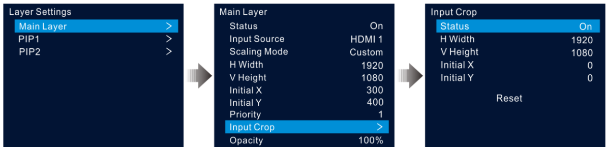
Figure 5-13 Input crop
