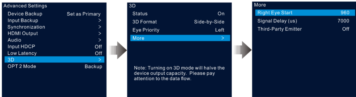
Figure 5-40 More Settings
