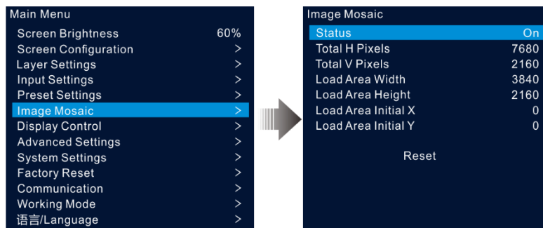
Figure 5-23 Image mosaic
