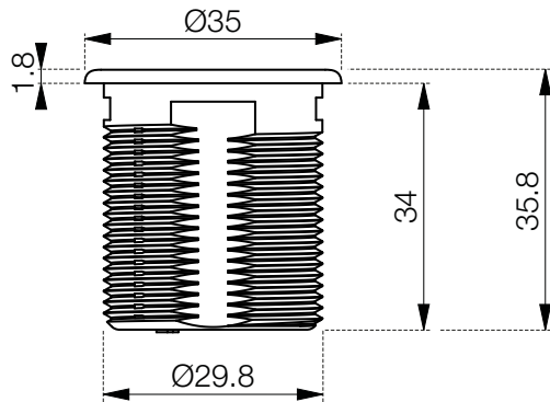
Front view (Grommet)
