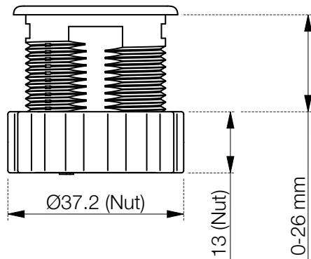
Front view (Grommet & nut)
