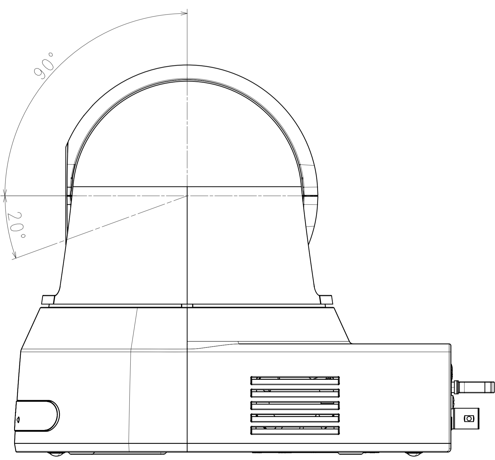
SIDE VIEW
